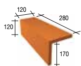
202 V17 Links linker gevelpan - 5 per lm - 2 kg
