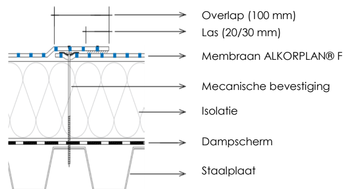
Fig. 8- Overlapverbindingen
